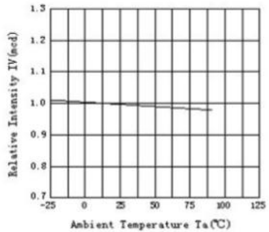
Relative Intensity vs. Ambient Temperature
