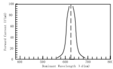
Luminous Spertun ( T_a=25^\circ\text{C} ) SPECTRAL RADIANCE
