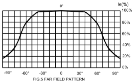
50% Power Angle: 145°
