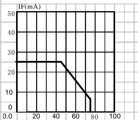
FIG.5 MAXIMUM FORWARD DC CURRENT VS AMBIENT TEMPERATURE(Tjmax=105)
