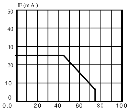
FIG.5 MAXIMUM FORWARD DC CURRENT VS AMBIENT TEMPERATURE (Tjmax=105 °C)
