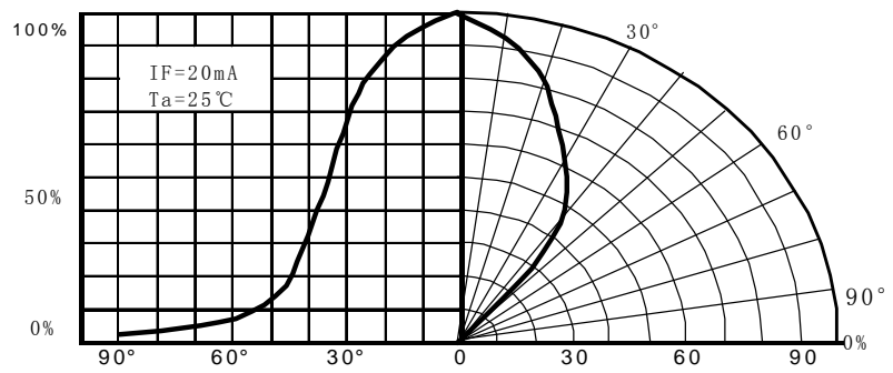
Fig.6 FAR FIELD PATTERN
