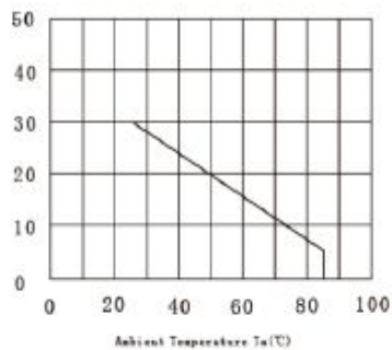
FORWARD CURRENT VS DERATING CURVE 正向电流随温度曲线图
