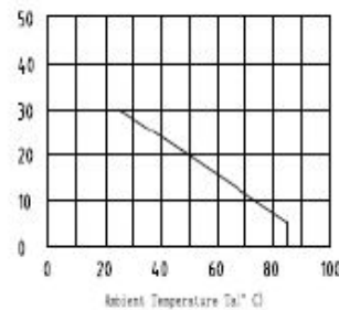
FORWARD CURRENT VS DEGRATING CURVE 正向电流随温度曲线图
