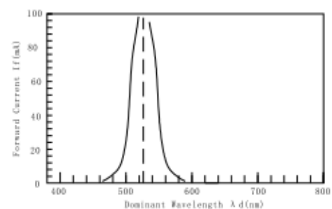
Luminous Spertum ( T_a=25^\circ\text{C} ) SPECTRAL RADIANCE
